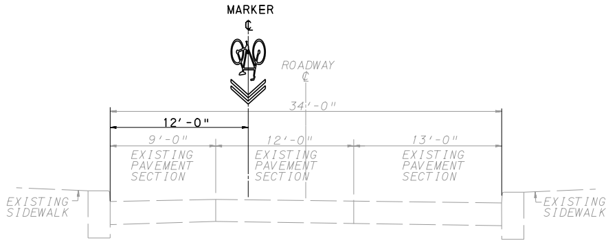
SHARED LANE MARKER LOCATION DETAIL SEE TC-8600 FOR MARKER DIMENSIONS MARKER TO BE PLACED 12' INSIDE RIGHT CURB SOUTHBOUND DIRECTION
