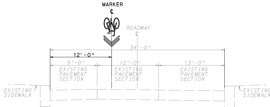
SHARED LANE MARKER LOCATION DETAIL SEE TC-8600 FOR MARKER DIMENSIONS MARKER TO BE PLACED 12' INSIDE RIGHT CURB SOUTHBOUND DIRECTION
